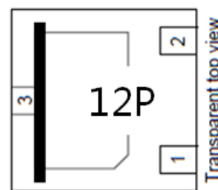
12P = Device Marking Code Bar denotes cathode
